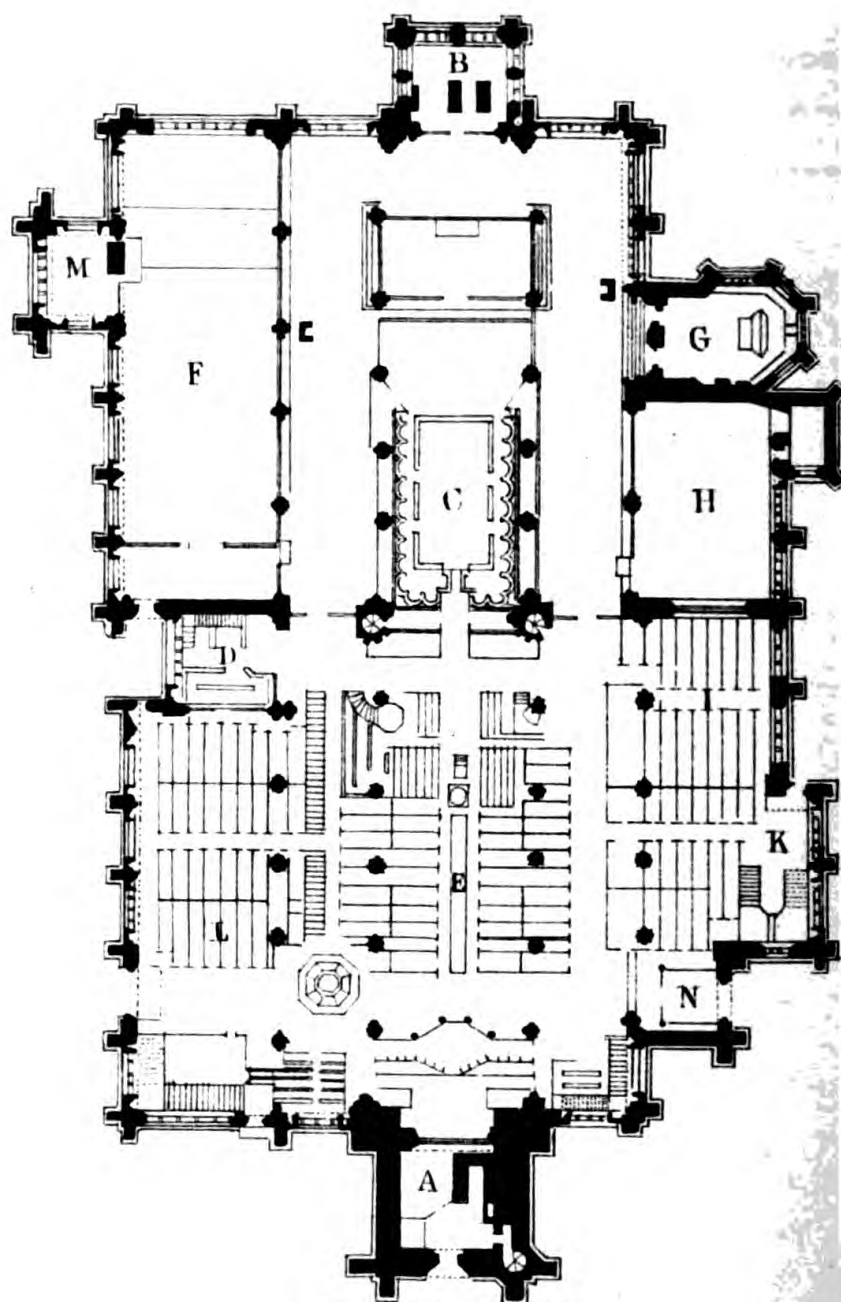
GROUND PLAN.
