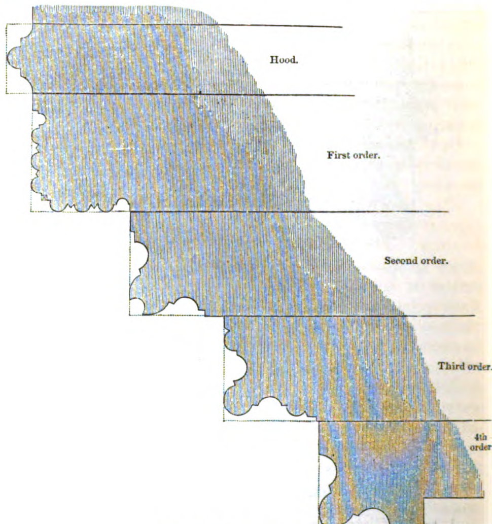
Arch mouldings of north doorway.
