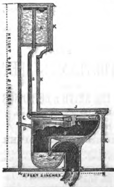
SECTION & PERSPECTIVE ELEVATION OF PATENT EXCELSIOR CABINET, W.C.
