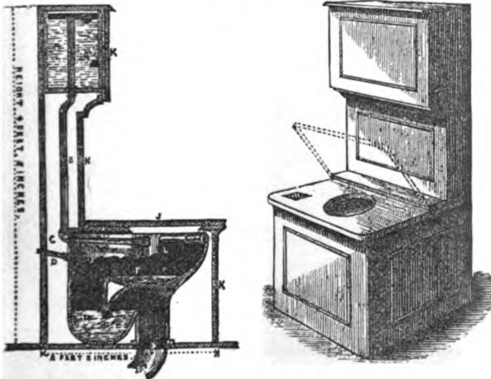
SECTION & PERSPECTIVE ELEVATION OF PATENT EXCELSIOR CABINET W. C.
