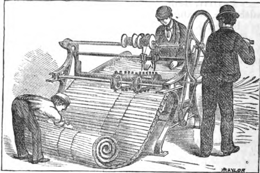
Machine at work. Capable of Producing 1,500 Feet per Hour.
